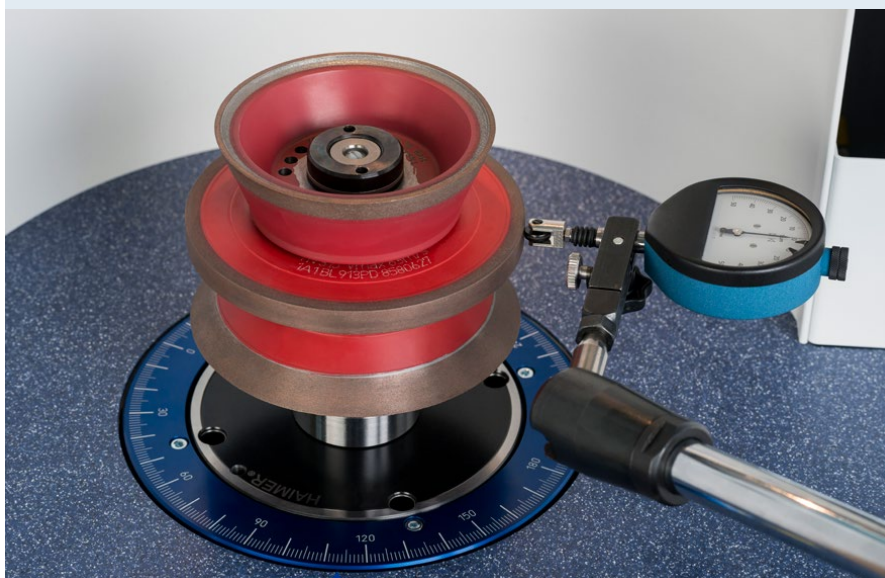
Runout measuring
