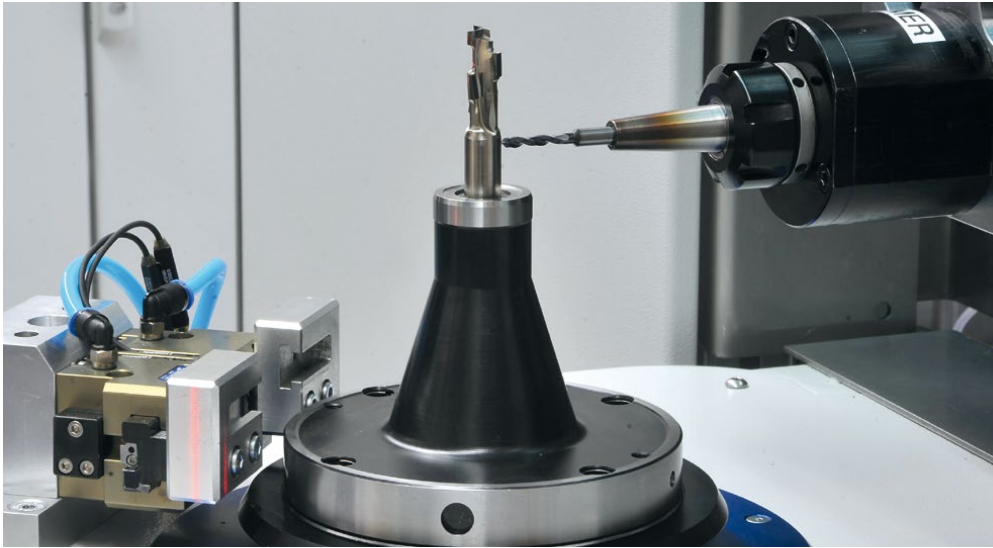
Balancing of tools with a HG balancing adapter for tools with a cylindrical shank For further information, please go to page 55.
