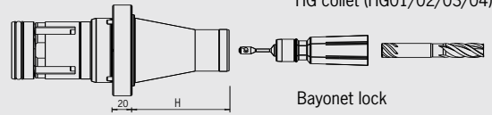
HG collet (HG01/02/03/04)
