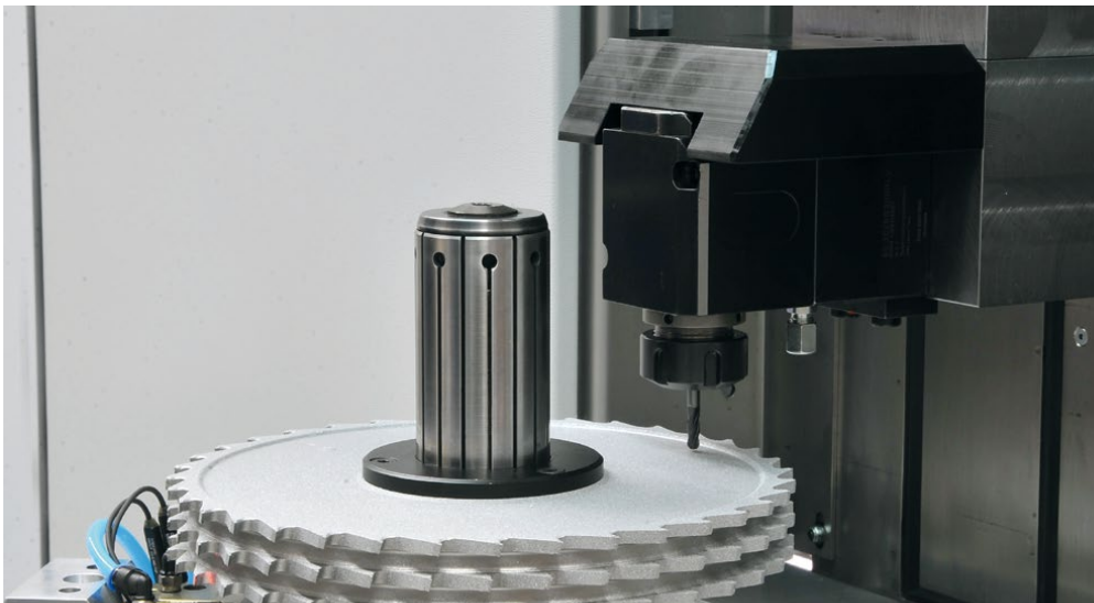
Balancing of PCD jointing cutters for laminate Balancing enables the best edge quality for the piece of furniture by vibration-free tool run. In addition, the noise while machining is reduced to a minimum.
